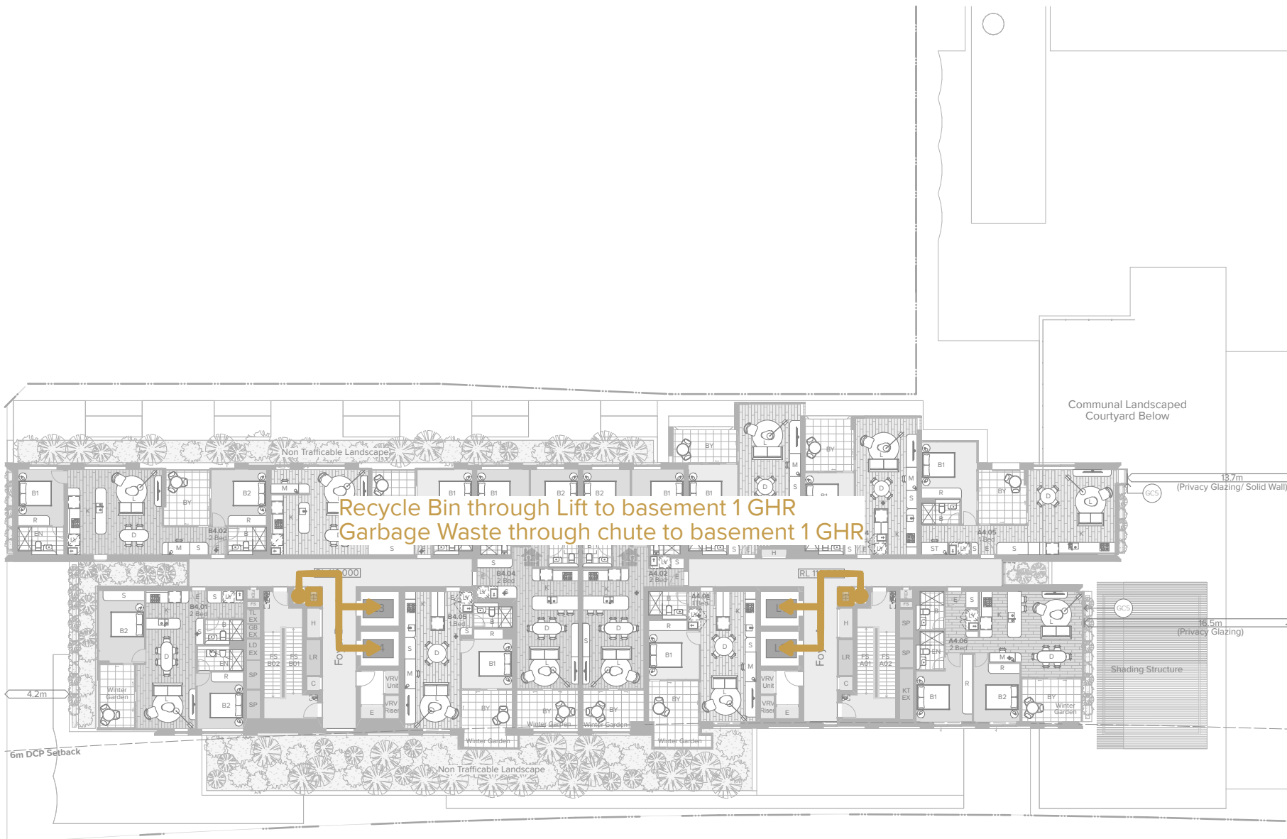
Level 04 - Level 19 (typical)
